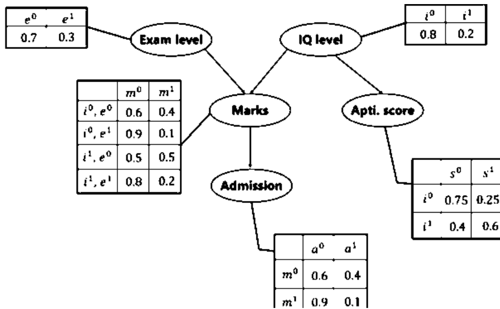
Figure 1: Bayesian Network
